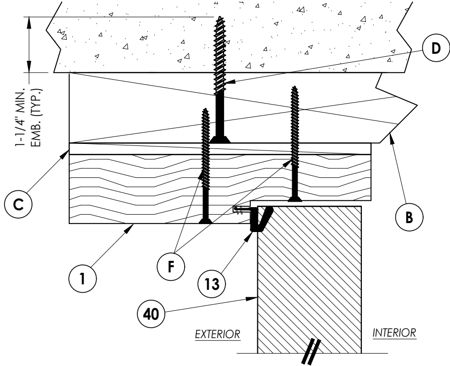
2 6 VERTICAL CROSS SECTION Inswing shown - outswing also approved
