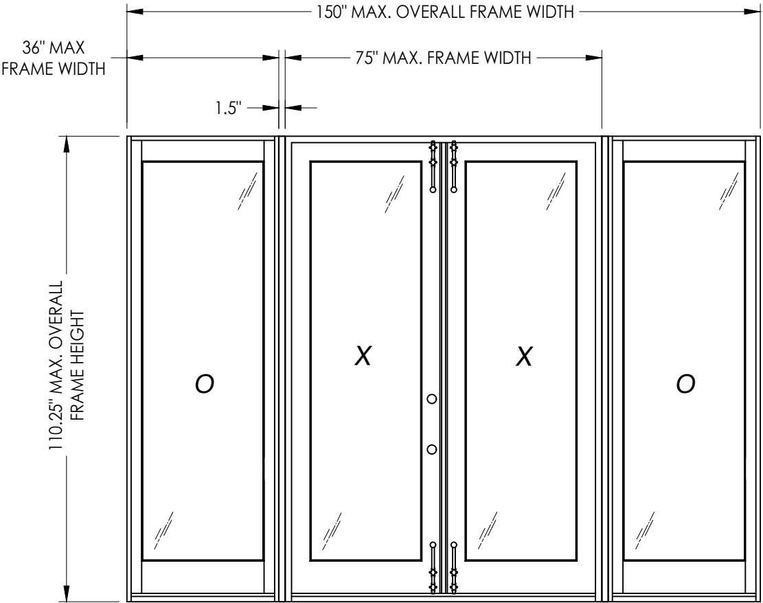
FULL GLAZED PANELS SHOWN
