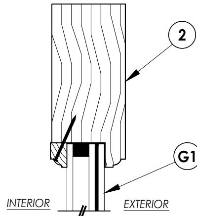
2/2 HORIZONTAL CROSS SECTION
