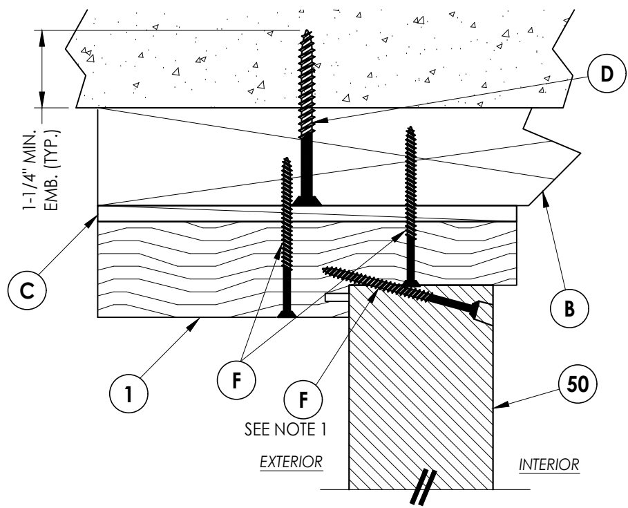
1 6 VERTICAL CROSS SECTION Inswing shown - outswing also approved
