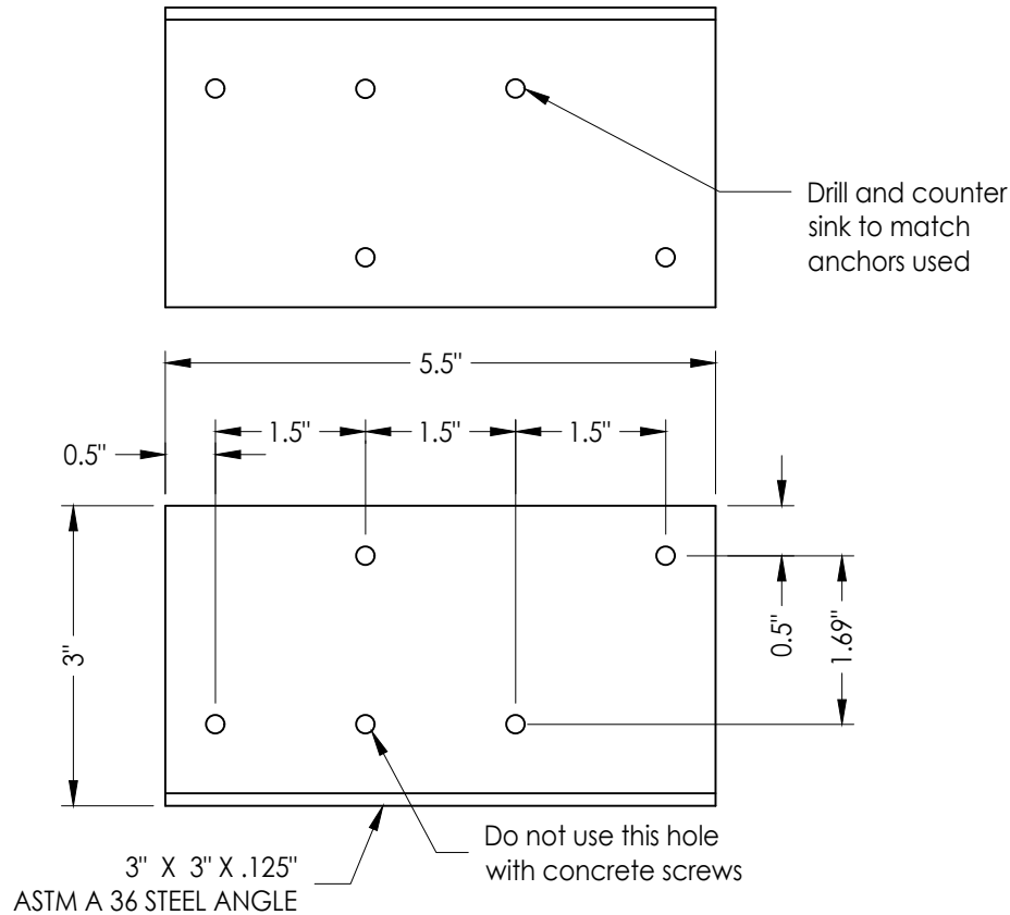
24 SUPPORT ANGLE
