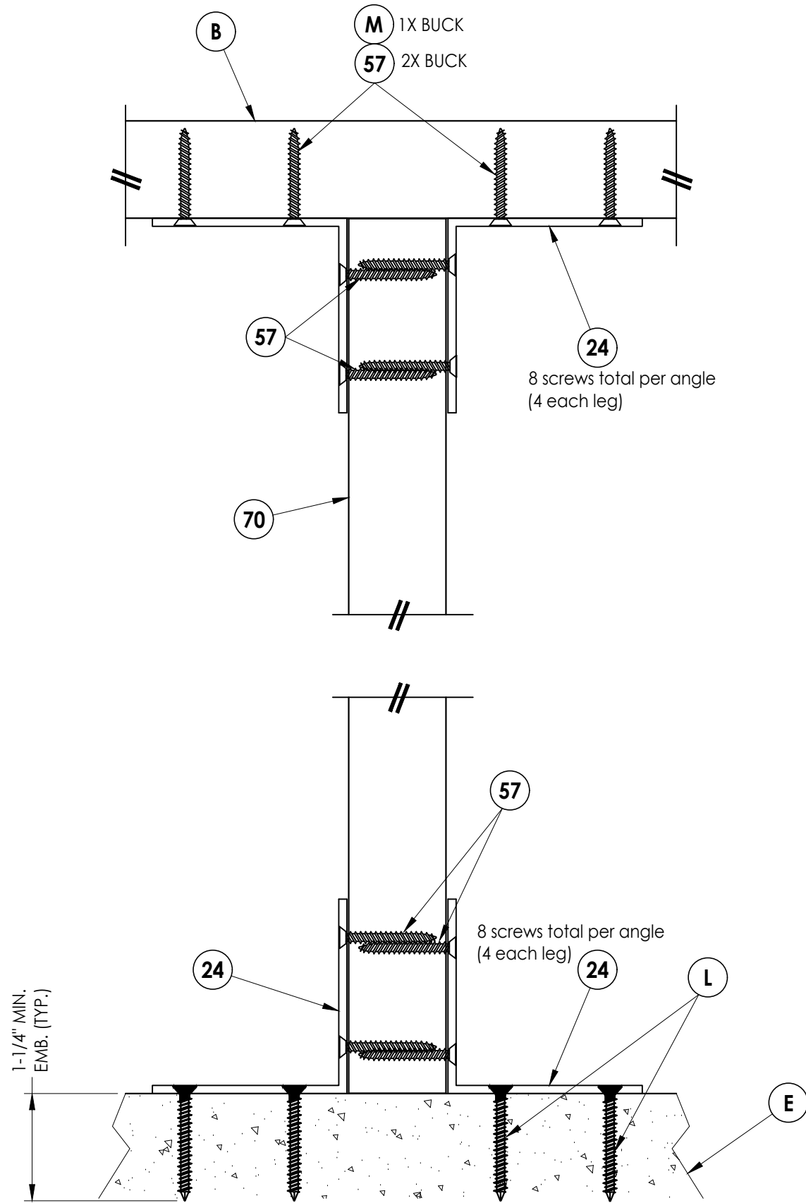
MULLION ANCHORING DETAIL
