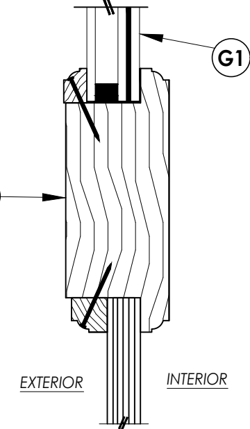
2/2 HORIZONTAL CROSS SECTION
