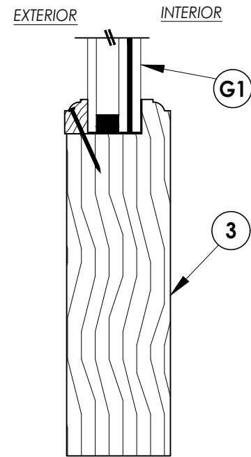
5/2 VERTICAL CROSS SECTION
