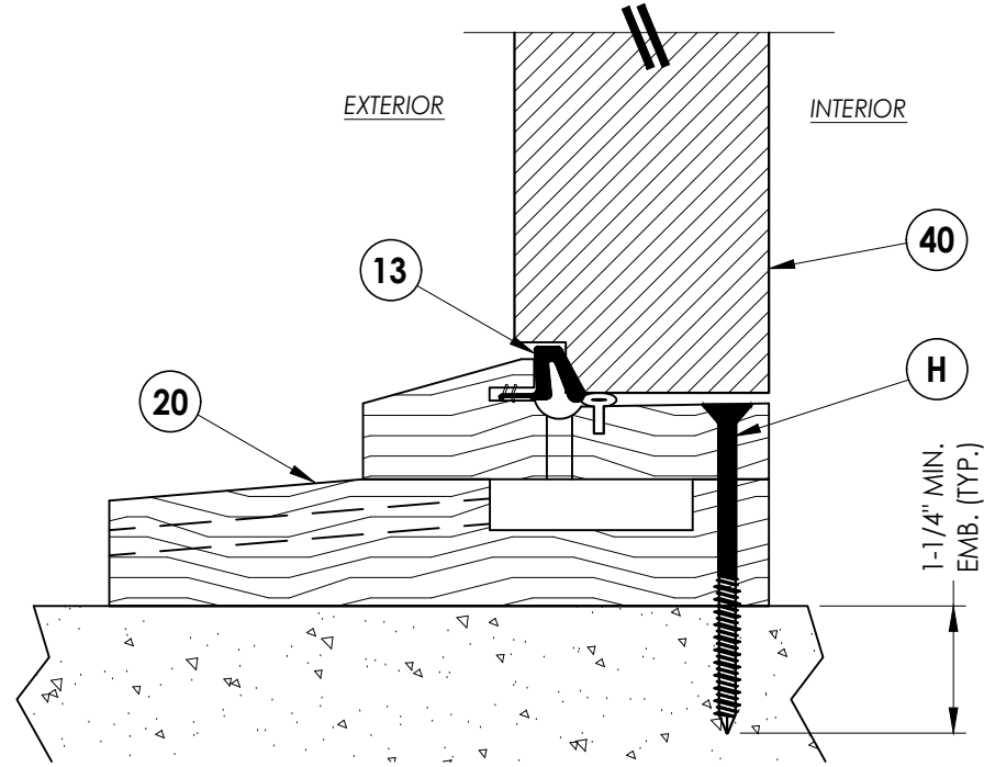
3 6 VERTICAL CROSS SECTION Inswing sill - door
