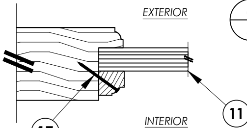
3/2 HORIZONTAL CROSS SECTION
